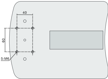
FIXTURE ATTACHMENT MOUNTING
