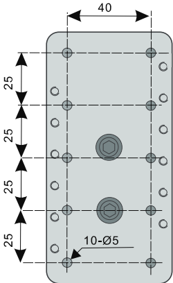
GAUGE MOUNTING PLATE
